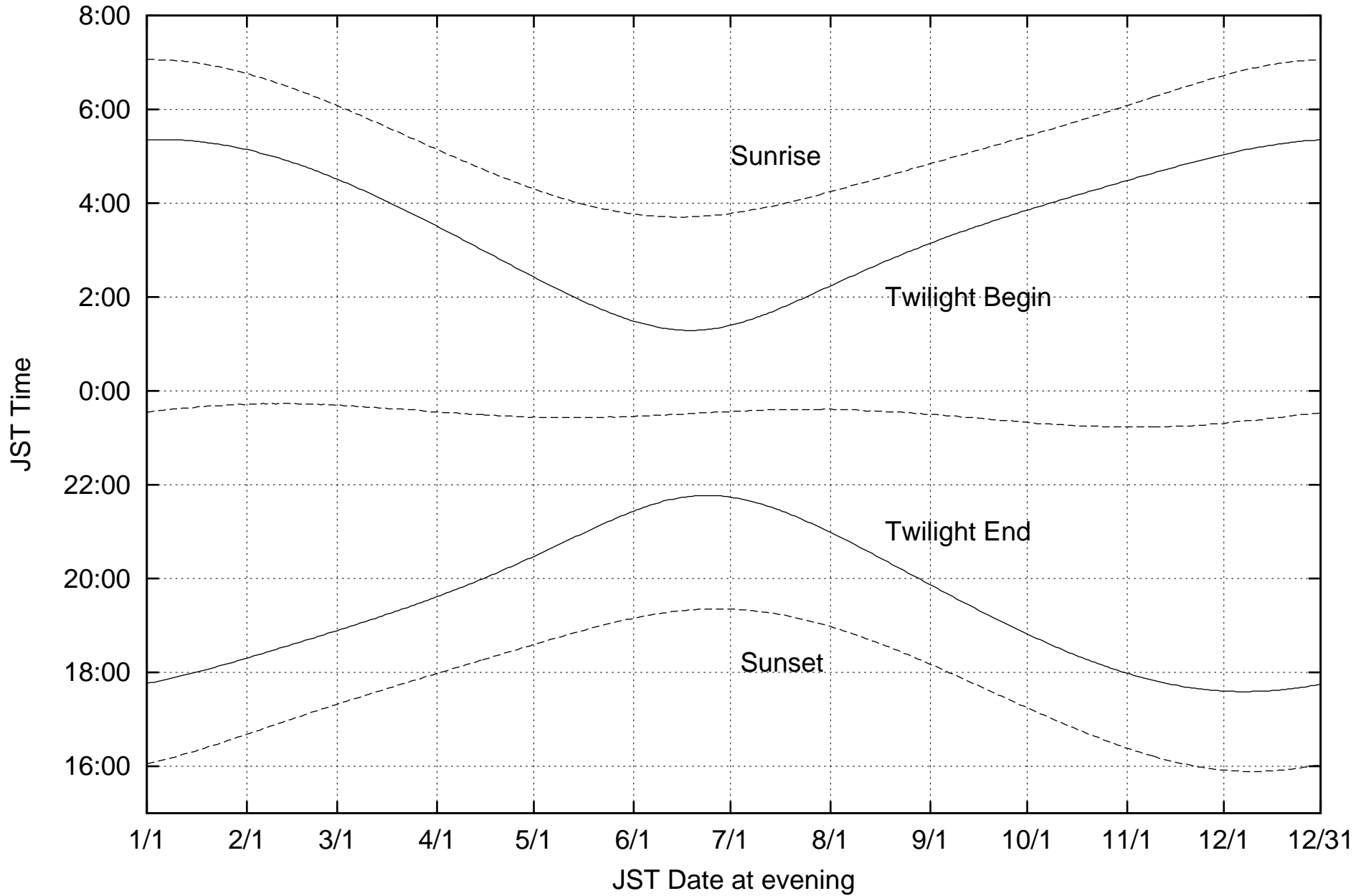
2011 Sunrise and Sunset times at Pirka Telescope
