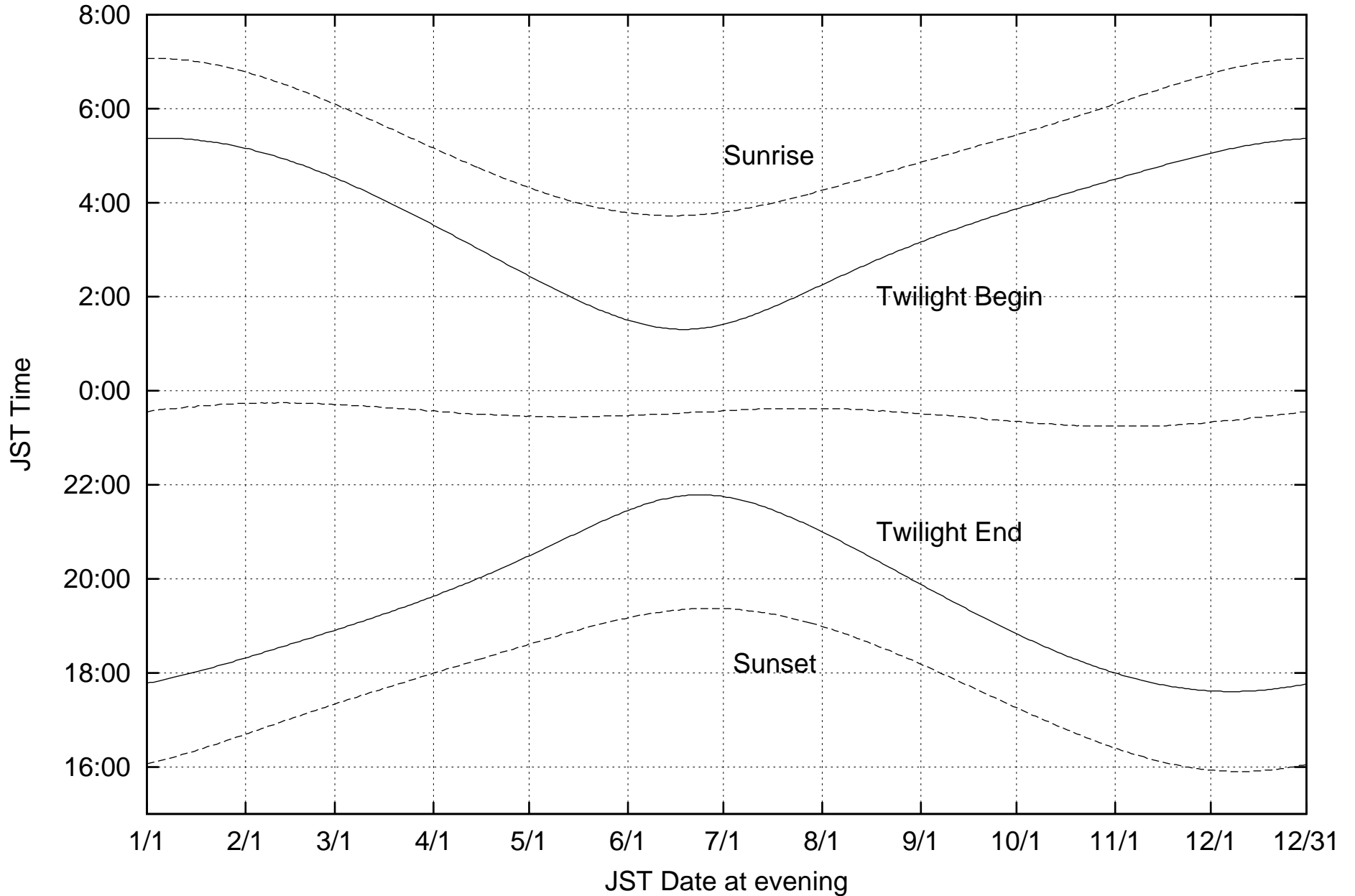
2015 Sunrise and Sunset times at Pirka Telescope
