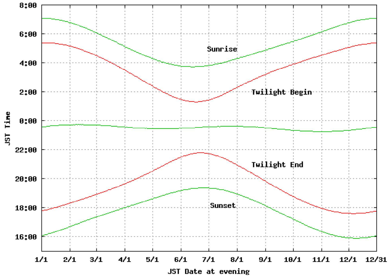
2018 Sunrise and Sunset times at Pirka Telescope
